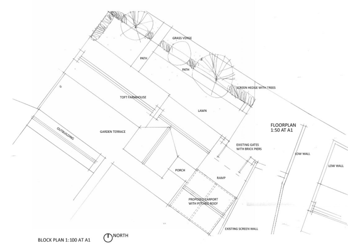
BLOCK PLAN 1:100 AT A1
