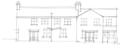
SOUTH ELEVATION, EXISTING 1:100 AT A1
