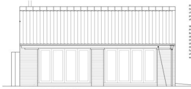
EAST ELEVATION, EXISTING 1:50 AT A1
