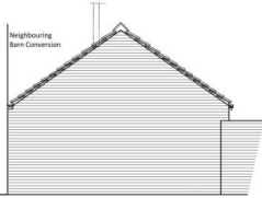
SOUTH ELEVATION, EXISTING 1:50 AT A1
