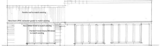
EAST ELEVATION, PROPOSED 1:50 AT A1
