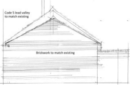
SOUTH ELEVATION, PROPOSED 1:50 AT A1
